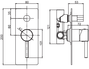
BL70DS Wall mixer with diverter Ø35mm Cartridge
