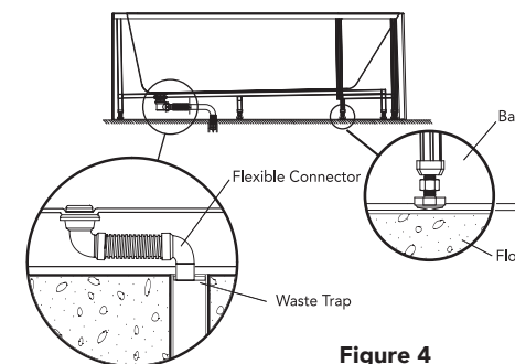
Figure 4 Flexi-Dinger installation
